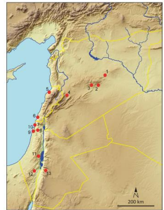
Fig. 5. Map showing the location of the Hummal site and other Palaeolithic sites with important blade components. 1 El Kowm (Hummal), 2 Jerf Ajla, 3 Duara Cave, 4 Yabrud, 5 Masloukh, 6 Adlun, 7 Hayonim, 8 Qesem, 9 Tabun, 10 Misliya Cave, 11 Abu Sif, 12 Rosh Ein Mor, 13 Ain Dilla. Map by R. Jagher.
