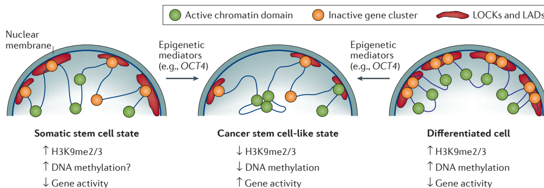
Figure 2 | Change in cell state towards cancer stem cell states induced by reprogramming of the 3D epigenome. This hypothetical scheme explains how epigenetic mediators (for example, OCT4 ) might reprogramme the epigenome to tip over normal somatic stem cells or differentiated progenitor cells into cancer stem cell states displaying phenotypic heterogeneity. Large organized chromatin K9 modifications (LOCKs) overlapping with lamina-associated domains (LADs) are hypothesized to be largely absent in somatic stem cells (left panel) to ensure epigenetic flexibility associated with the multipotent state. The coordination of cell-type-specific repressed states (right panel) within the LOCKs/LADs is facilitated by epigenetic modifiers establishing multiple layers of epigenetic modifications, such as H3K9me2, H3K9me3, and DNA methylation. The localization of LOCKs/LADs to the lamina leads to the separation of active and inactive domains to reduce transcriptional noise and to provide barriers for dedifferentiation. Conversely, the unscheduled activation of epigenetic mediators leads to the erosion of LADs/LOCKs and the emergence of hypomethylated blocks during the neoplastic process. This, in turn, induces phenotypic heterogeneity by increasing the variability in expression and the probability of switches between the diverse cellular states within the tumour. A loss of LOCKs is postulated, moreover, to interfere with the constraints of enhancer–promoter communication within and between topologically associated domains (TADs), enabling the clustering of oncogenic super-enhancers and expression domains (green circles) to coordinate the expression of oncogenic pathway members (centre panel).
