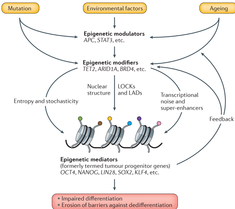
Figure 1 | Functional classification of cancer genes and their contribution to malignancy. Ageing, inflammation and chronic exposure to carcinogens impinge on epigenetic modulators, such as adenomatous polyposis coli ( APC ) and signal transducer and activator of transcription 3 ( STAT3 ), that fine tune and regulate the function of epigenetic modifiers — for example, TET methylcytosine dioxygenase 2 ( TET2 ) and AT-rich interaction domain 1A ( ARID1A ) — to bring about changes in the expression of epigenetic mediators — for example, sex-determining Y-box 2 ( SOX2 ) and OCT4 — whose gene products regulate developmental potential. Chronic exposure to a fluctuating, cancer-predisposing environment and ageing promote the selection for epigenetic heterogeneity in vulnerable populations of somatic stem cells and progenitor compartments. Mutations in modulators and modifiers are often selected for during cancer development, which leads not only to increased cell proliferation, but also to the unscheduled expression of mediators that, in turn, inhibit differentiation and promote epigenetic plasticity by affecting the epigenetic modulators and modifiers in a feedback loop. The mechanism of epigenetic instability involves the erosion of barriers against dedifferentiation, such as large organized chromatin K9 modifications (LOCKS) overlapping with lamina-associated domains (LADs), and the emergence of hypomethylated blocks that contain the most variably expressed domains of the tumour genome and interfere with normal differentiation. Increased transcriptional noise at developmentally regulated genes is paralleled by the redistribution of super-enhancers from cell-fate-determining genes to oncogenes that further stabilize the cancer cell state. Stochastic changes in unstable chromatin states lead to the continuous regeneration of epigenetic heterogeneity that manifests as increased cellular entropy and provides the basis for the selection of the fittest during cancer evolution. BRD4 , bromodomain containing 4; KLF4 , Kruppel-like factor 4.
