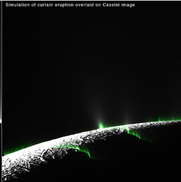
Simulation of curtain eruption overlaid on Cassini image
