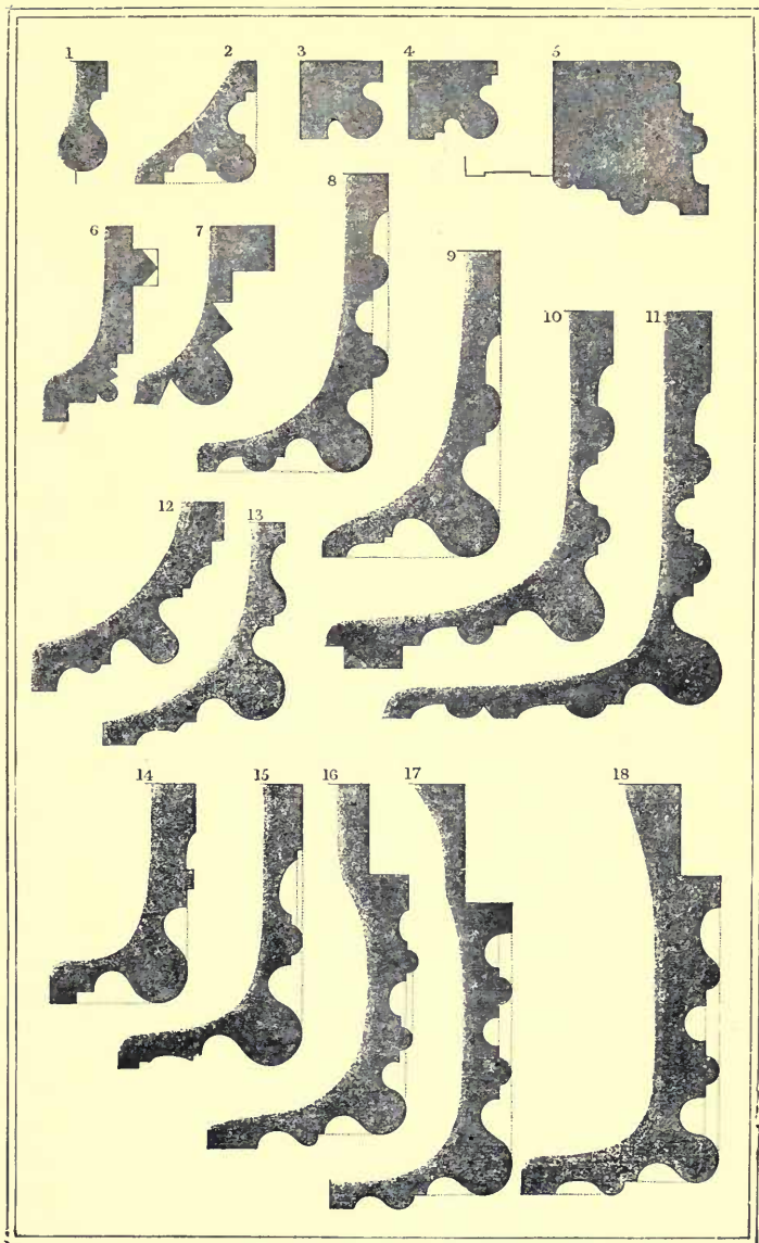
PLATE VI.—BYZANTINE JAMBS.
