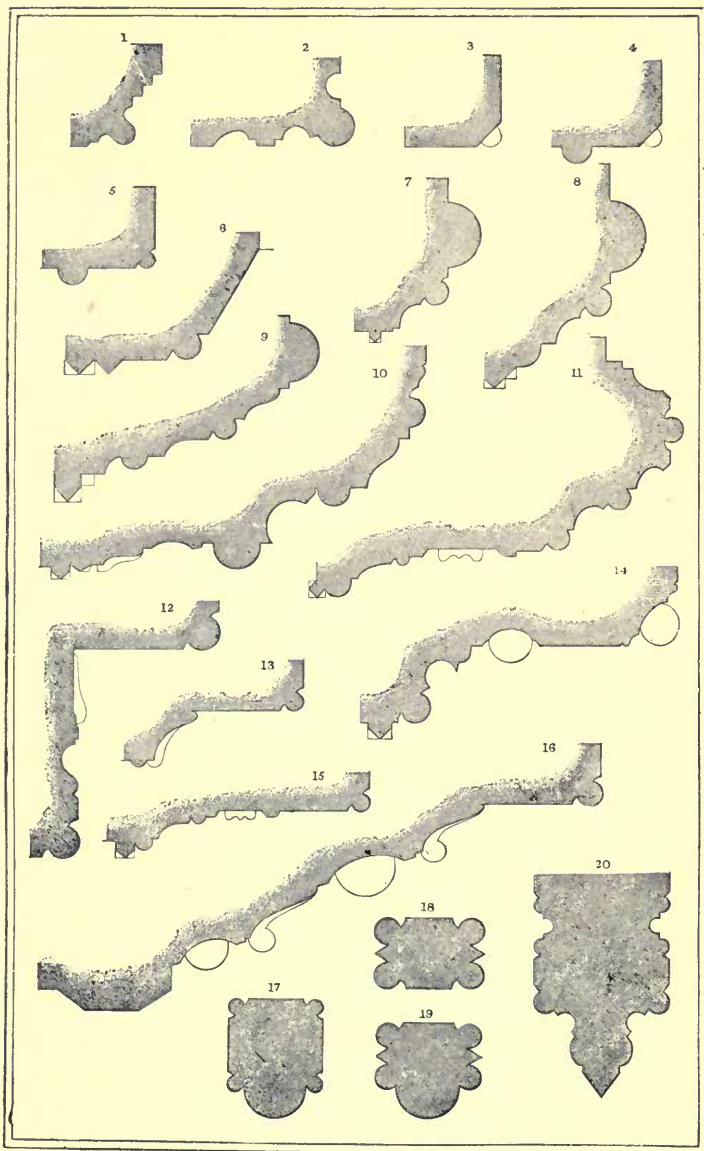
PLATE VII.—GOTHIC JAMBS.
