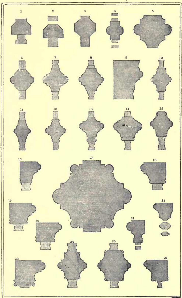
PLATE XI.—TRACERY BARS.
