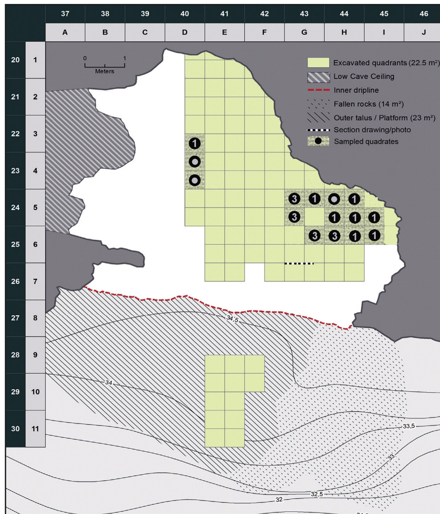
Fig. 2. Layout and stratigraphy of Blombos Cave. Layers sampled for tortoise analysis and total NISP for each sample are indicated. Sampled areas of the cave are indicated, with a “1” where only M1 deposits were sampled, a “3” where only M3 deposits were sampled, and a filled circle where both were sampled.
