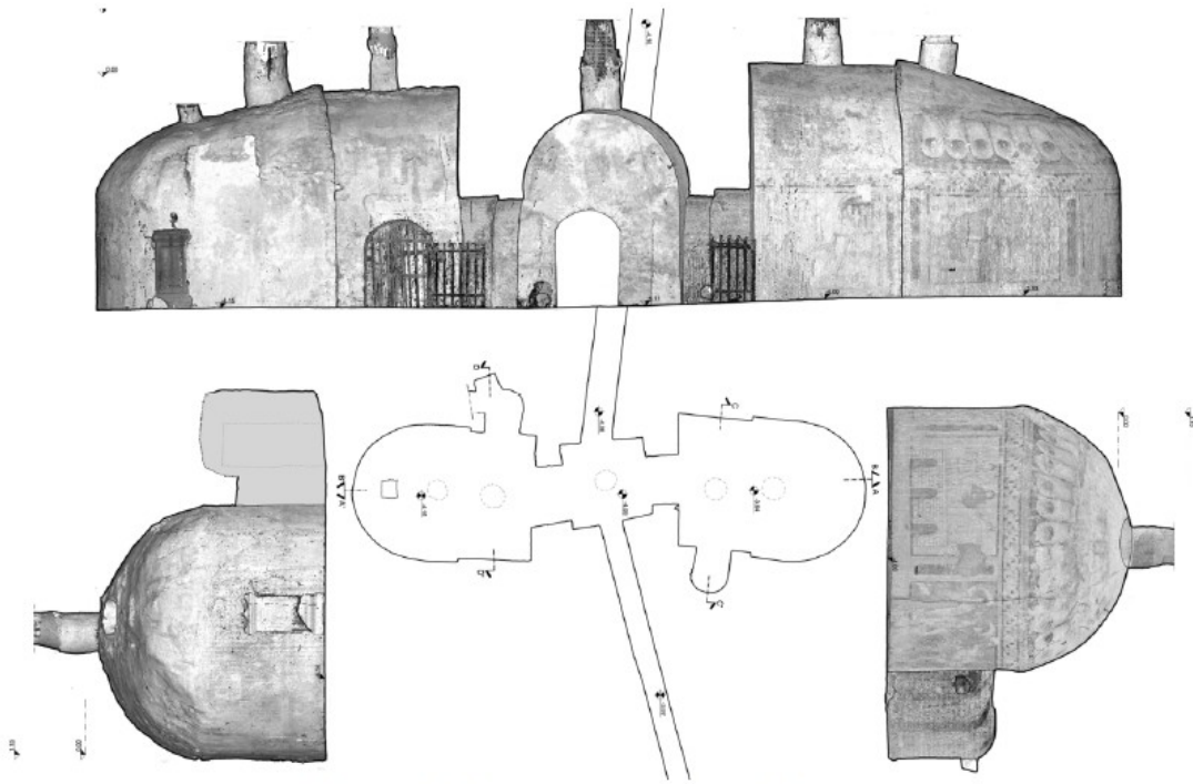
Figure 2: Plan view and elevations rendered with point cloud image in gray scale.
