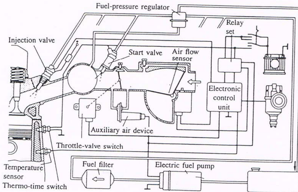
FIGURE 7-12 Electronic multipoint port fuel-injection system with air-flow meter: Bosch L-Jetronic system. 9 (Courtesy Robert Bosch GmbH and SAE.)
