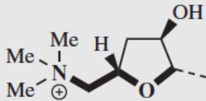
muscarine
