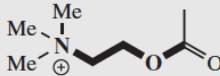
acetylcholine
