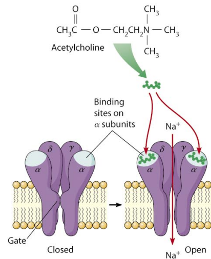
(c) Function of receptor
