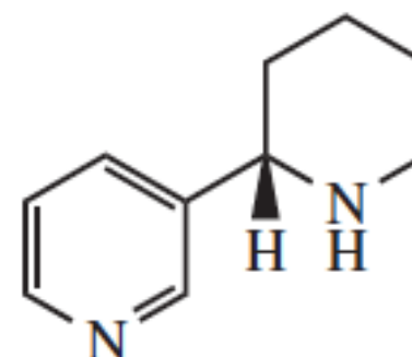
anabasine
