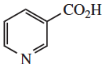
nicotinic acid (niacin/vitamin B 3 )
