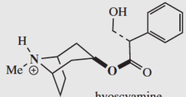
hyoscyamine (shown as conjugate acid)
