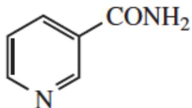
nicotinamide
