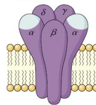
(b) Structure of receptor
