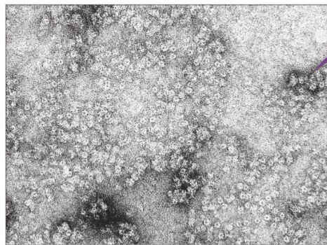
(a) Acetylcholine receptors in electroplex membrane
