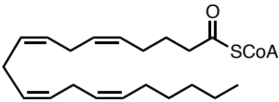
Ac Arachidonico 20:4 (5c, 8c, 11c, 14c)
