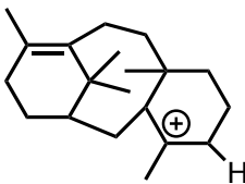
Catione Taxenile
