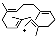
GGPP Carbocatione
