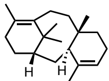
Taxadiene
