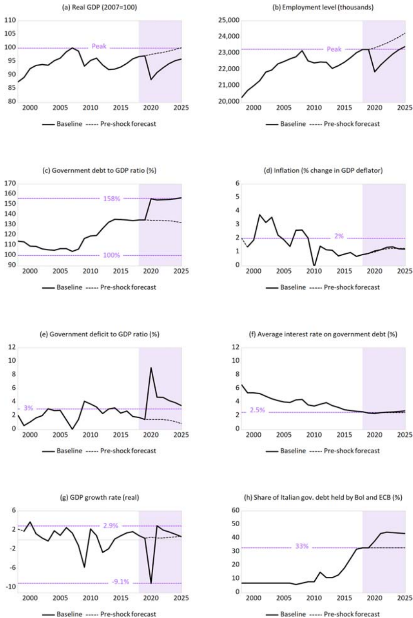
Figure 1. Observed series (1995–2019) and out-of-sample predictions (2020–2025): selected variables. Notes: shaded areas show the forecasted series.
