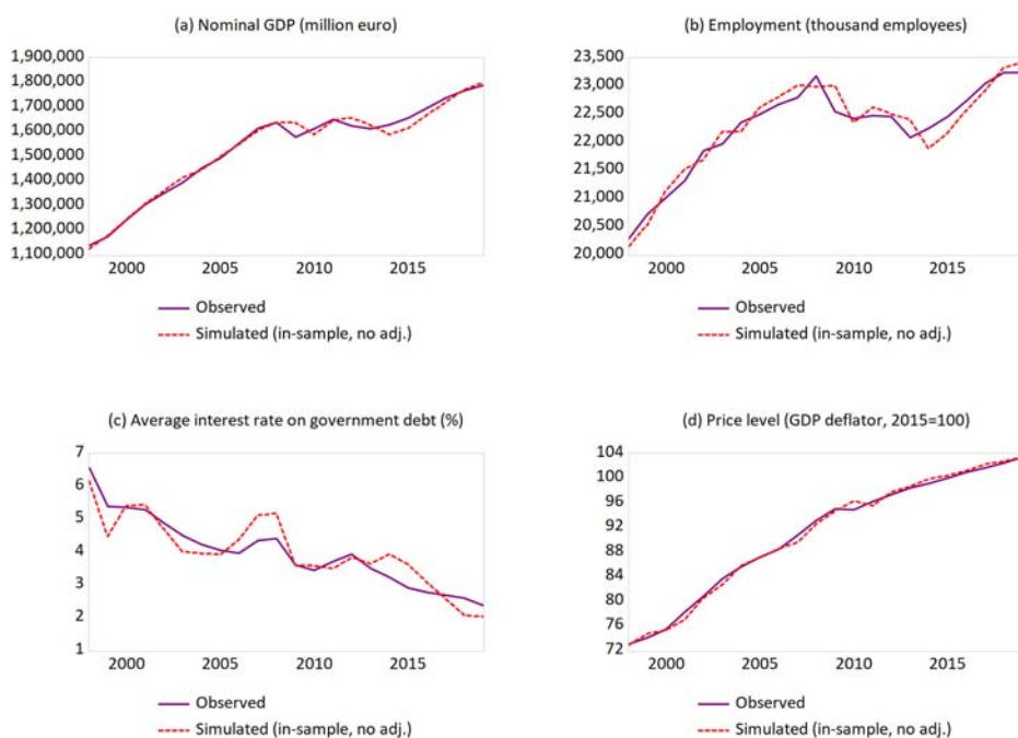
Figure A1. In-sample predictions: selected variables.
