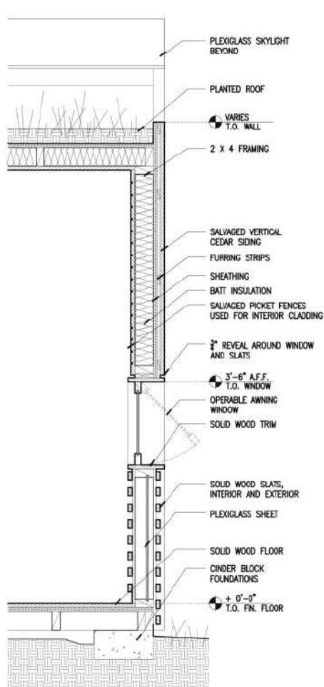
1 WALL SECTION AT WINDOW
