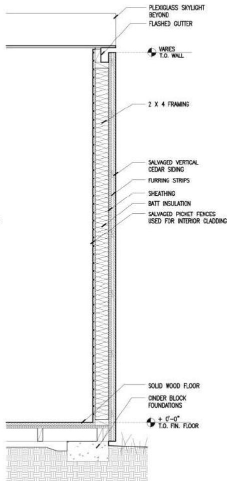
2 WALL SECTION
