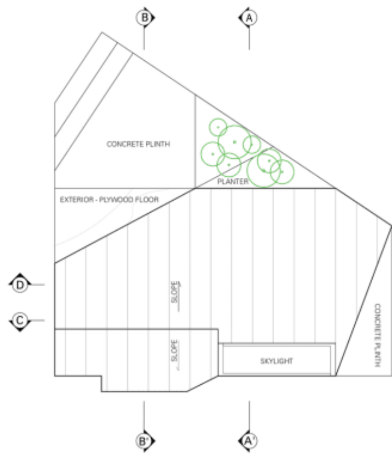
ROOF PLAN
