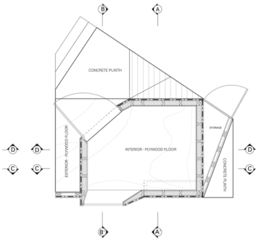
FLOOR PLAN
